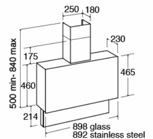
Line drawing includes the optional chimney accessory (code: AEC02SS)
